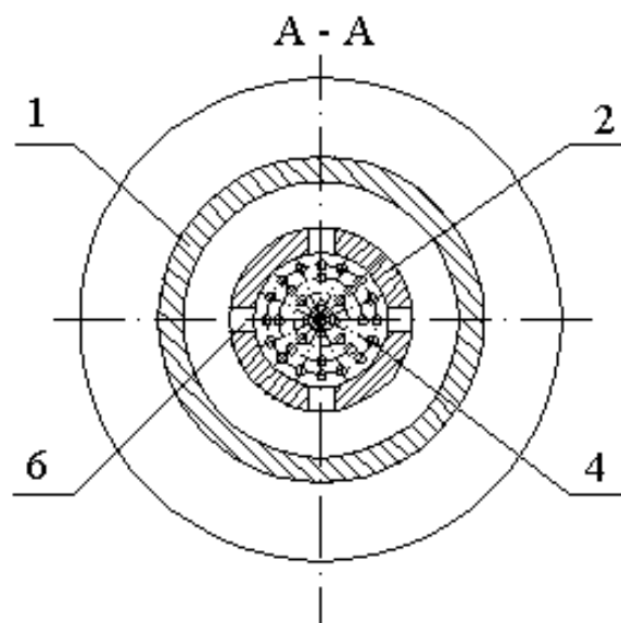
Figure 2 – Cross-section A – A of the mine gas pipeline fire stopper
